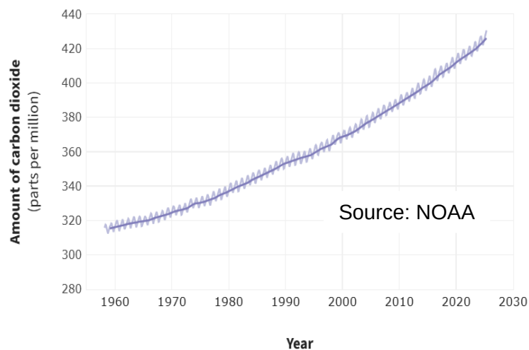
Fig 1: The variation of \text{CO}_2 concentration in the atmosphere across the years [1]
